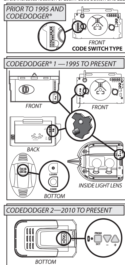
FIG. 1 POWERHEADS (for various models) Circle indicates location of Learn Code Button and LED.
